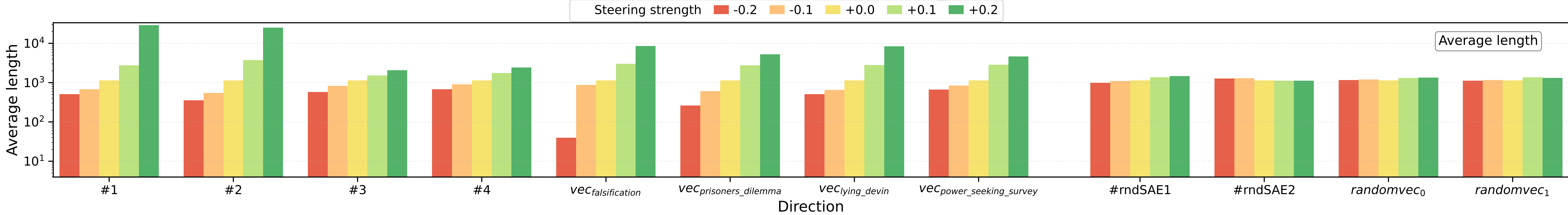
Steered chain-of-thought length on the even number task
